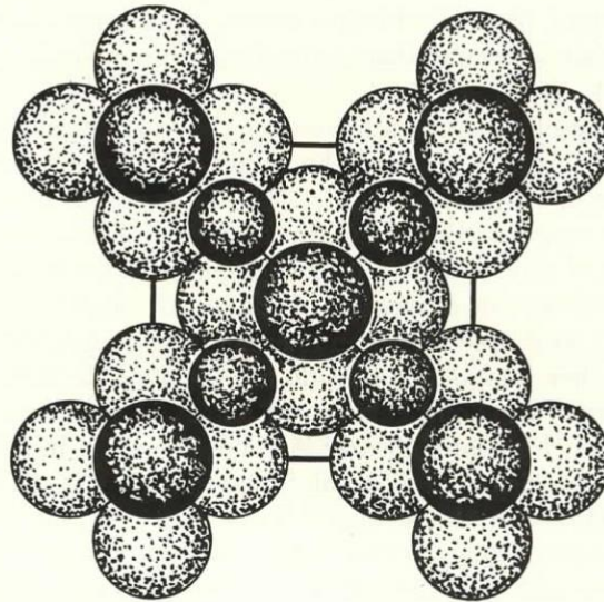
Fig. IXC,10a (top). The cubic K_2PtCl_6 structure projected along a cube axis.
